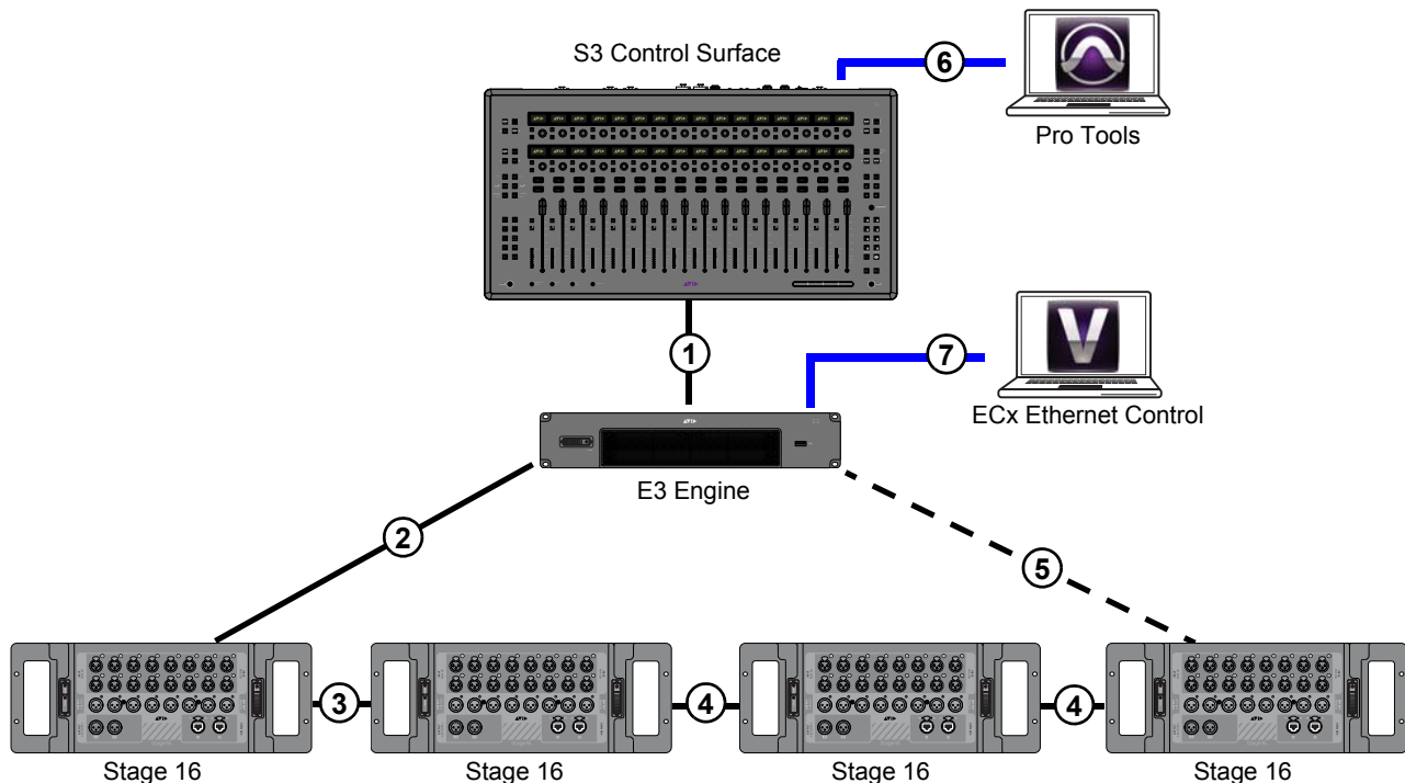
A basic S3L-X system
