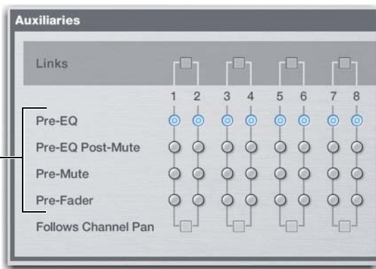
Aux bus pickoff points
