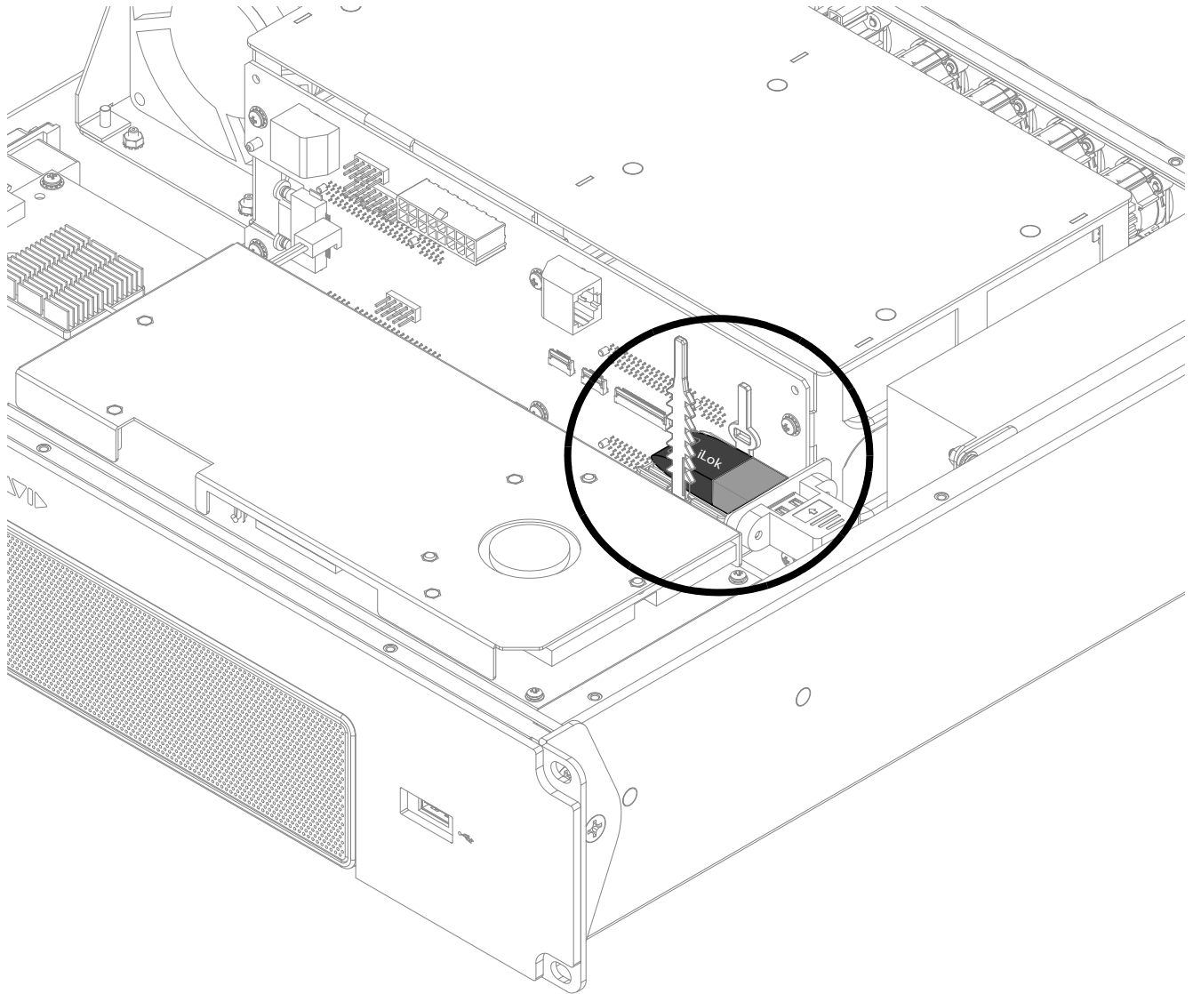
Interior of the E3 engine showing an attached iLok
