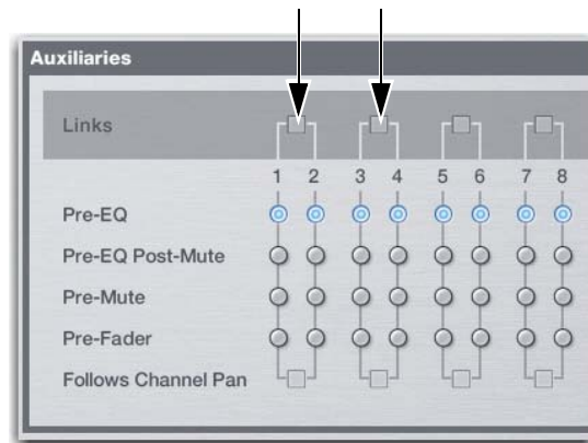
Bus pair checkboxes in the Options > Busses page
